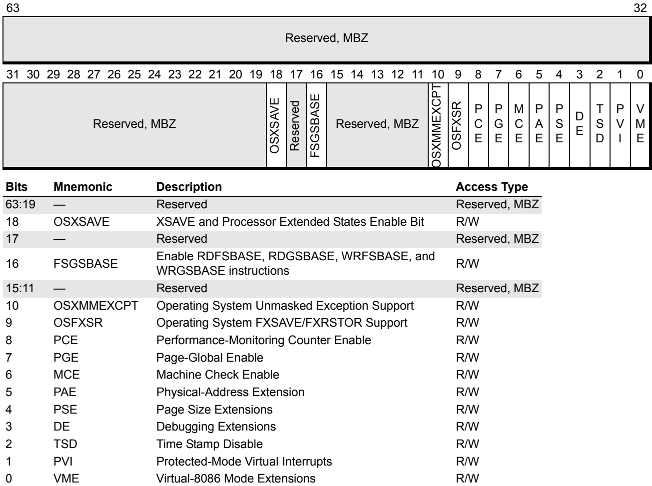
Figure 3-7. Control Register 4 (CR4)
