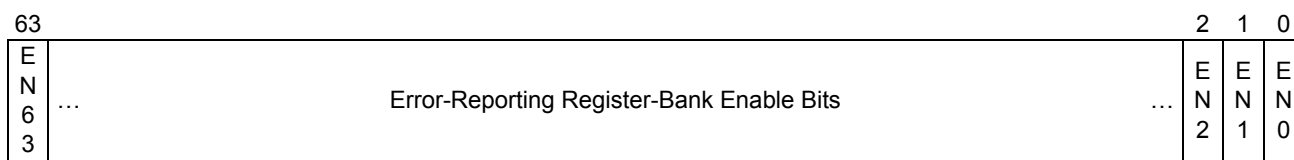
Figure 9-5. MCi\_CTL Register
