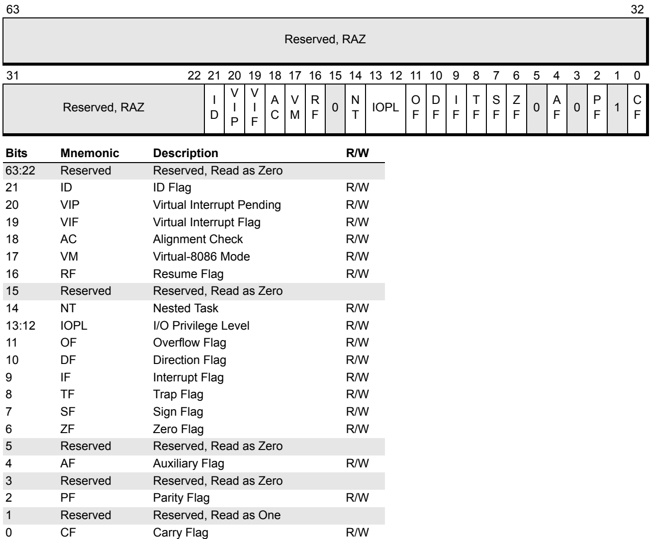
Figure 3-8. RFLAGS Register
