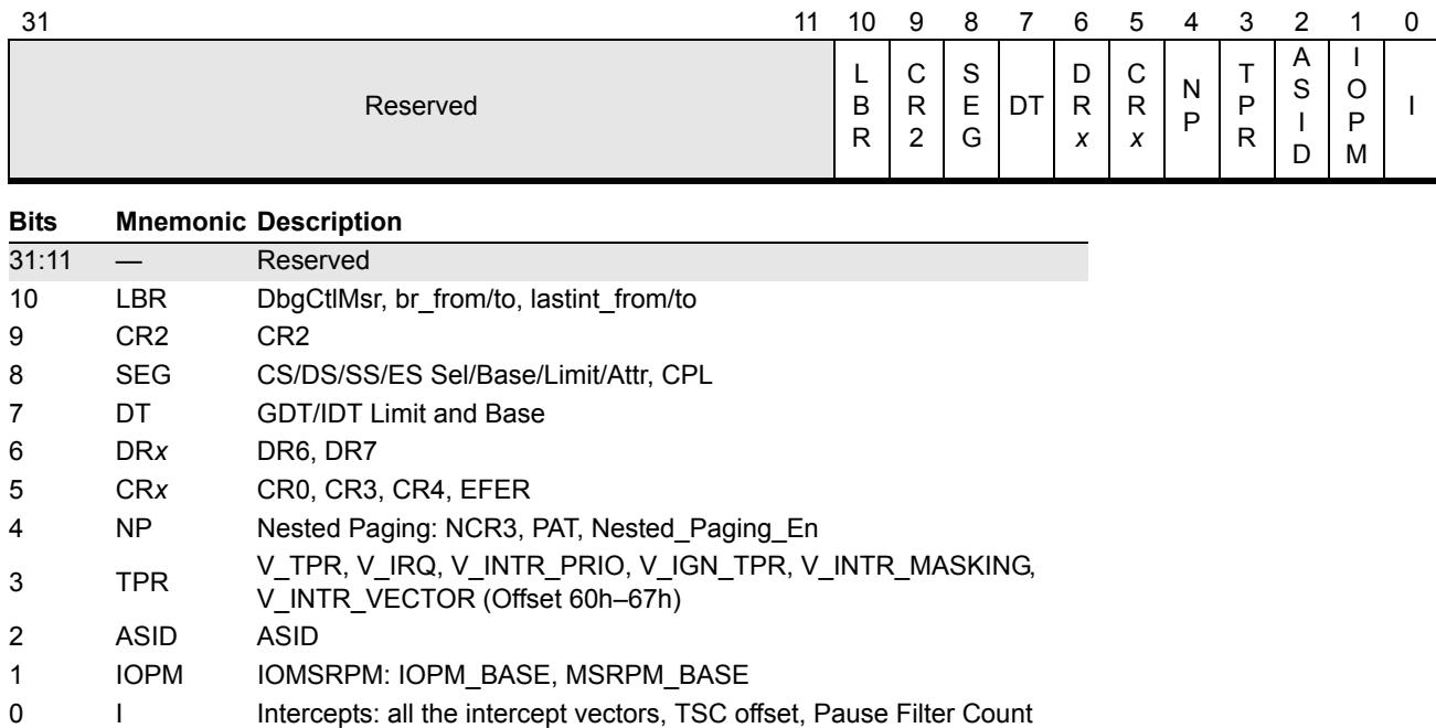
Figure 15-4. Layout of VMCB Clean Field
