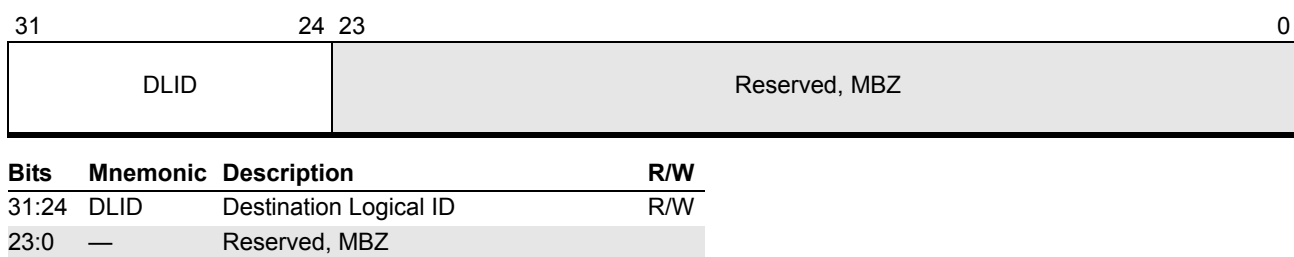
Figure 16-20. Logical Destination Register (APIC Offset D0h)
