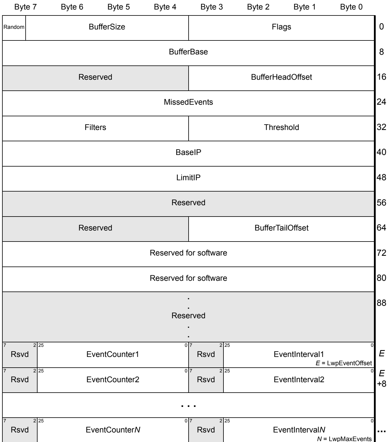
Figure 13-29. LWPCB—Lightweight Profiling Control Block
