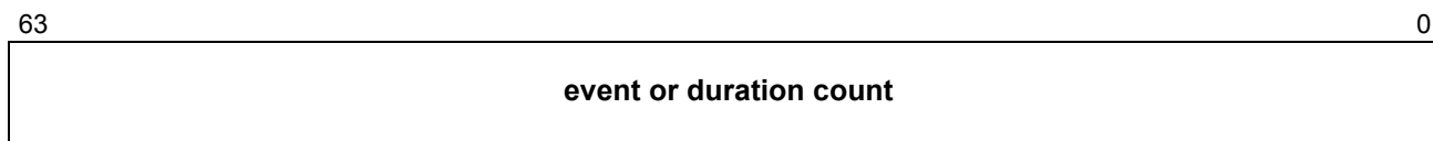
Figure 13-6. Core or NB Performance Counter
