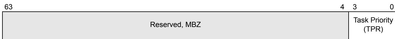
Figure 8-4. Task Priority Register (CR8)
