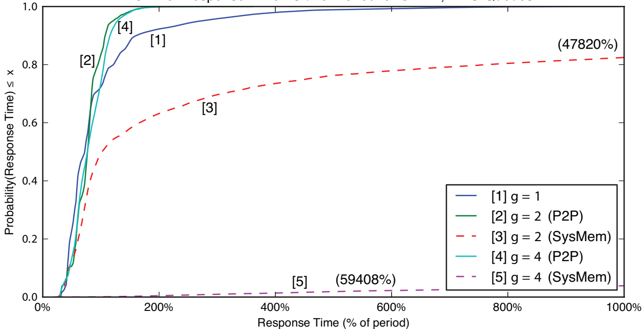
CDF of Response Time As % of Period for C-EDF, FIFO Queues
