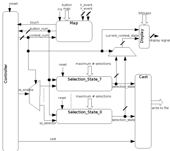
Figure 3: Design of the voting machine.
